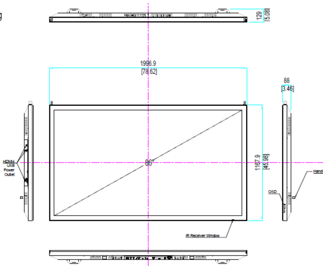
Front Drawing
