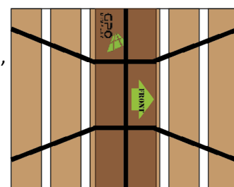
[Fig.3] Top View of strapping on a single display.
