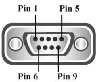
RS232 Pinout (9 Pin Male)
