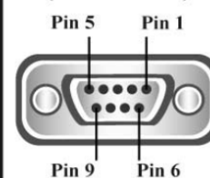
RS232 Pinout (9 Pin Female)
