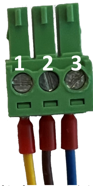
[Fig. 7] RS232 terminal with wires inserted
