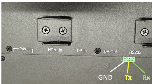
[Fig. 5] Rear view of display
