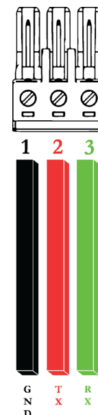
[Fig. 7] RS232 terminal with wires inserted
